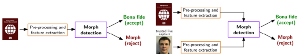
Figure 2: Morphing attack detection scenarios. Left: Single image Morphing Attack Detection, Right: Differential Morphing Attack Detection (image source: Hochschule Darmstadt).
