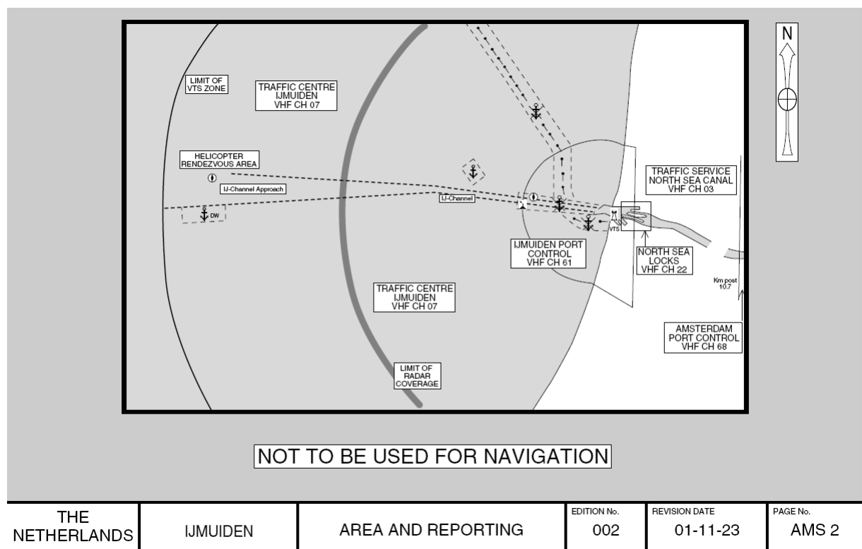
Figure 1. Example of the information from the World VTS Guide showing a.o. VTS radar coverage.
